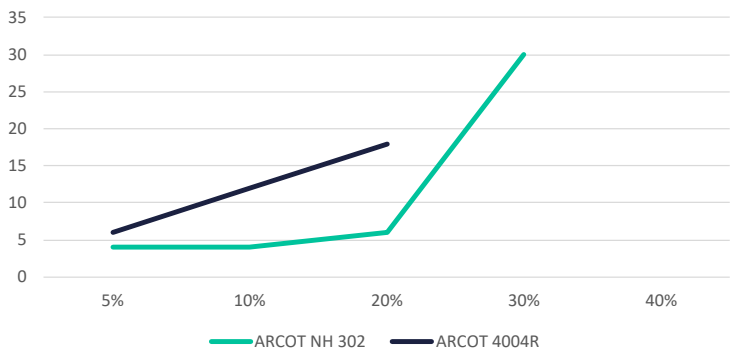
Salt Spray test in D60 solvent in hours (ASTM B 117)
