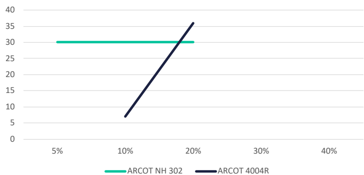
Salt Spray test in SN100 mineral oil in hours (ASTM B 117)
